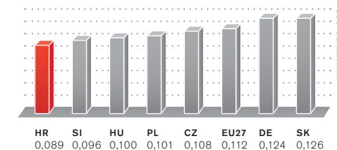
ELECTRICITY PRICES FOR INDUSTRIAL CONSUMERS €/kWh
